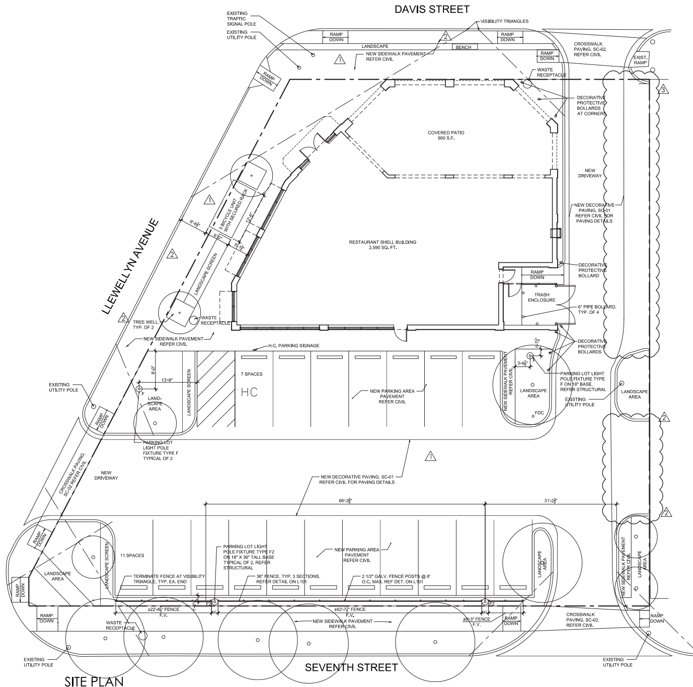
SITE PLAN
